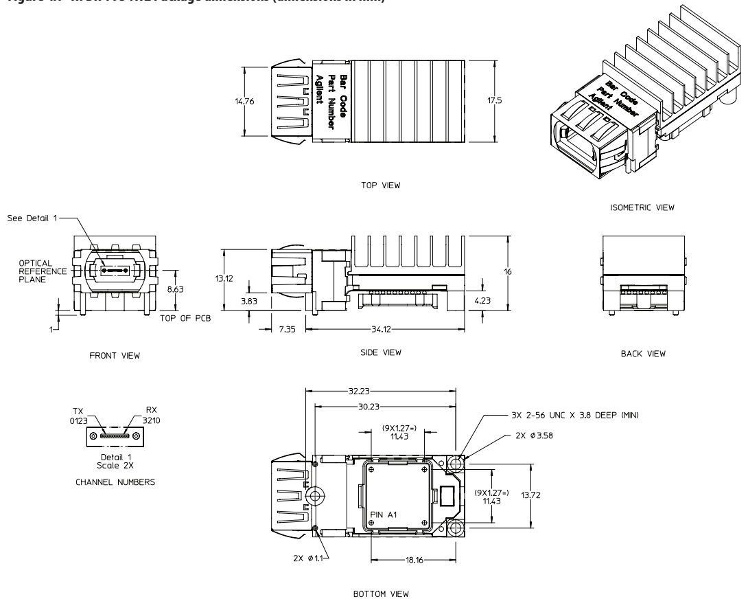
Figure 4B - HFBR-7934EWZ Package dimensions (dimensions in mm)
